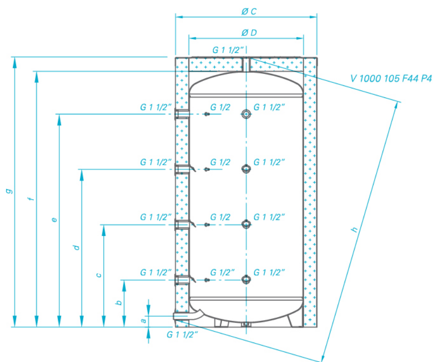
Dimensions [mm ± 5]
